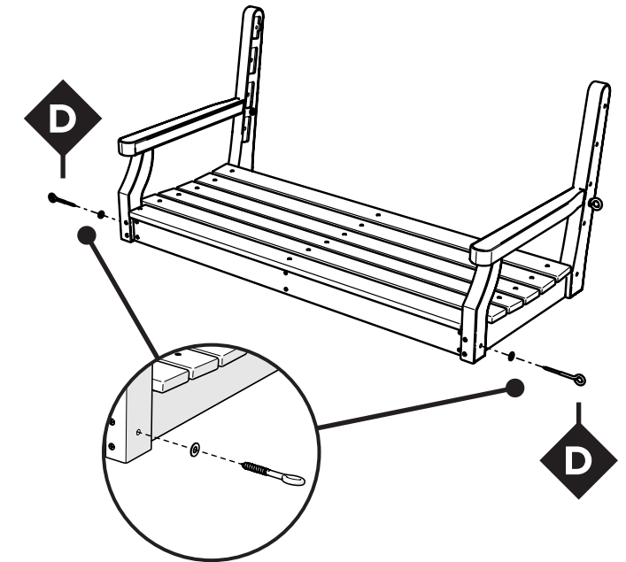
Washer
