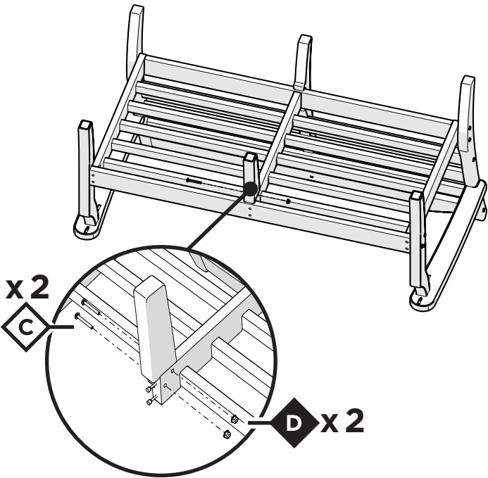
1.875" Fine Thread Bolt H.25-20X1.875
