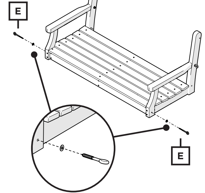
x2 Washer
